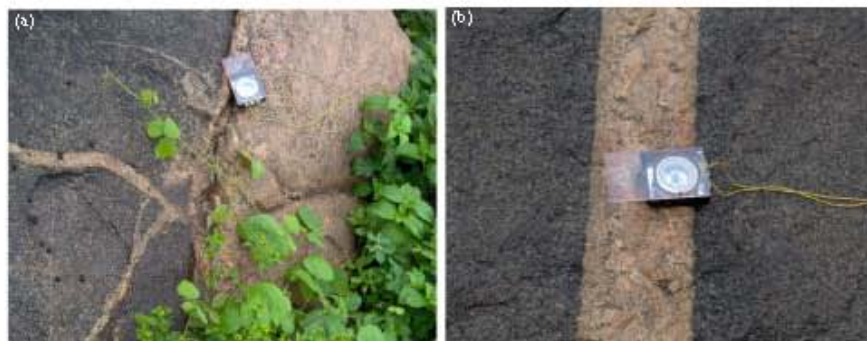
Fig. 2: (a) N-S, E-W, NNE-SSW trending pegmatite veins in charnockitic rock and (b) pegmatite vein cutting through an outcrop of the charnockitic rock
