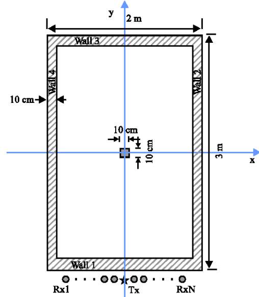
Fig. 1: TWIR measurement model configuration
