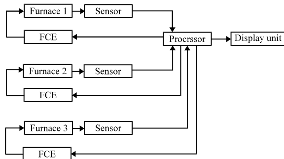
Fig. 1: Block diagram of a multiple furnace control system
