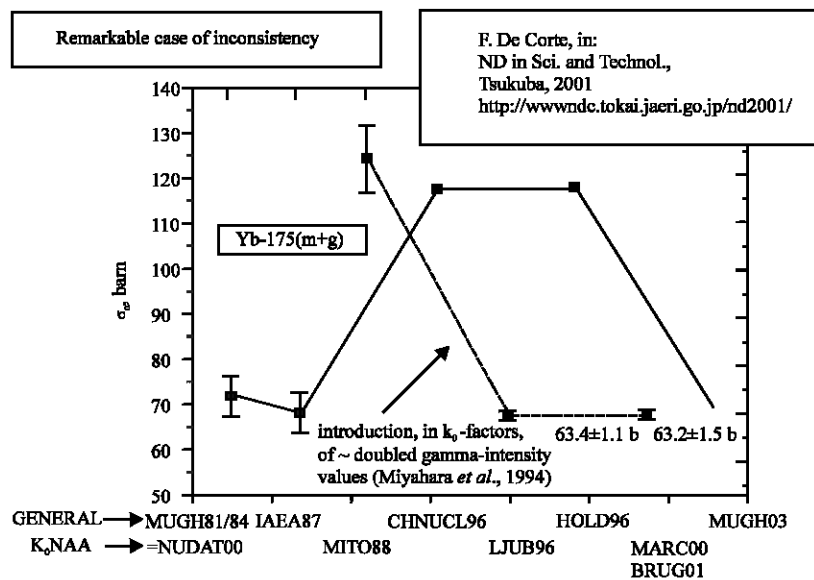
Fig. 1: Variations of Yb-175 thermal cross-section values
