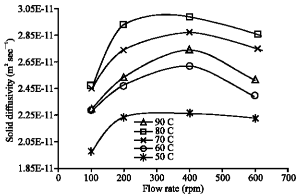
Fig. 5: Solid diffusivity, D_s , against flow rate
