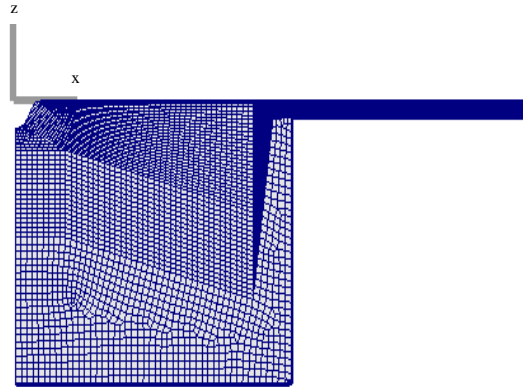
Fig. 1: Two-dimensional grid of the modeled engine
