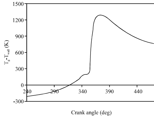
Fig. 12: Mean temperature difference between cylinder gas and inner wall surface
