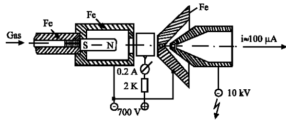
Fig. 1: The cold cathode Ion source with magnetic hollow cathode in cathode circuit
