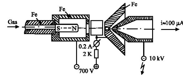
Fig. 2: Cold cathode Ion source with magnetic hollow cathode in anode circuit
