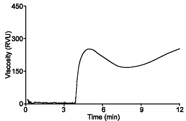
Fig. 2: RVA Pasting Curve of Red Cocoyam Cormels Starch
