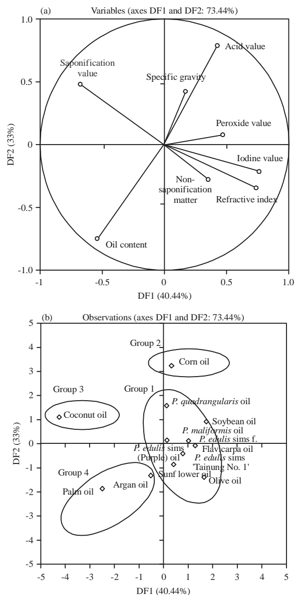
Fig. 1(a-b): (a) Plot of physicochemical properties of Passiflora seed oils and other commercial edible seed oils. The percentage in parentheses represents the variation in each component. (b) Positions of PC score of 12 seed oils analysed according to PC1 and PC2
