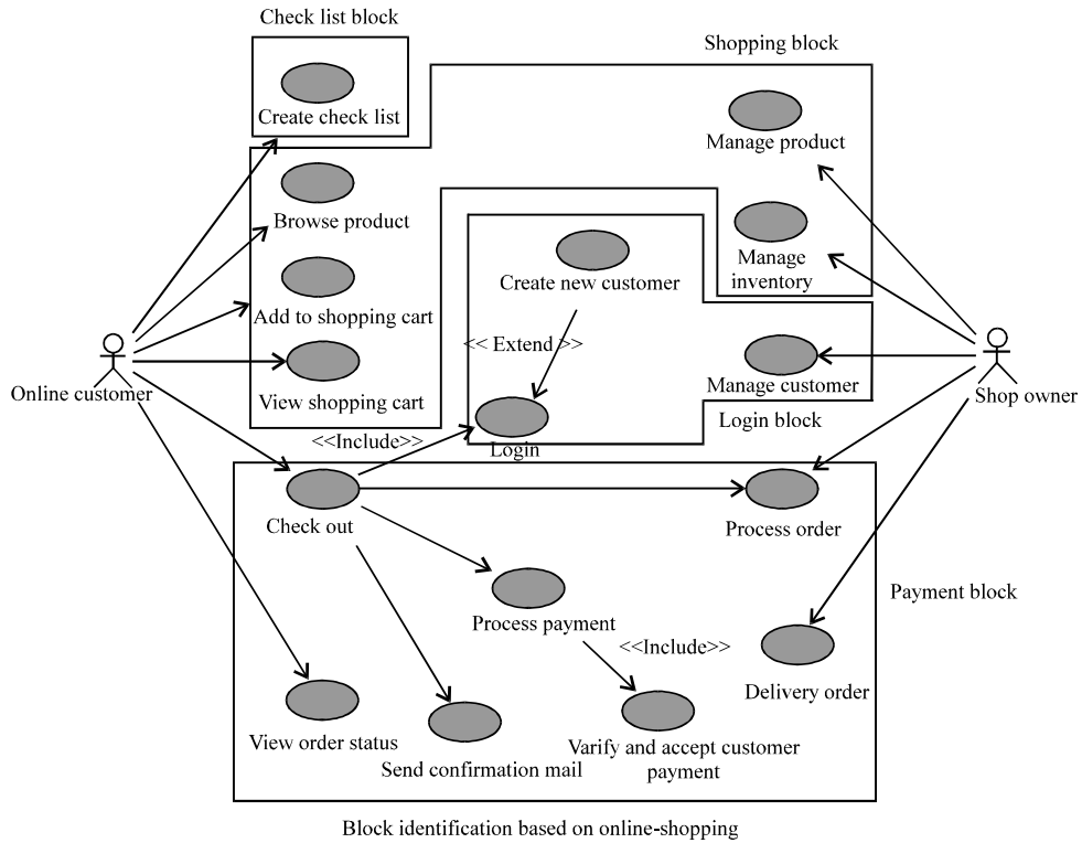
Fig. 6: Blocks identification
