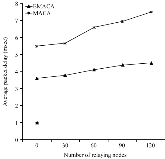
Fig. 5: Packet delay
