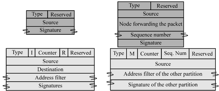
Fig. 3: Messages of FAP for initialization, joining node and partition merging procedure
