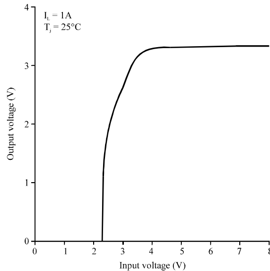
Fig. 2: Characteristics of voltage behavior (LM3940) ( http://www.ti.com/lit/ds/sym/links/lm3940.pdf )
