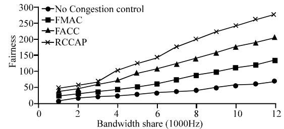
Fig. 8: Comparison of fairness metrics
