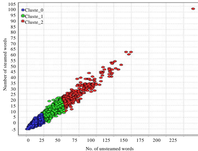
Fig. 3: Clustering with K-means visualization
