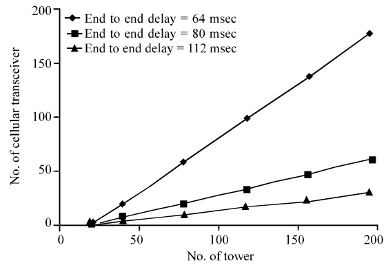
Fig. 7: Deployment of cellular transceiver for various size of network
