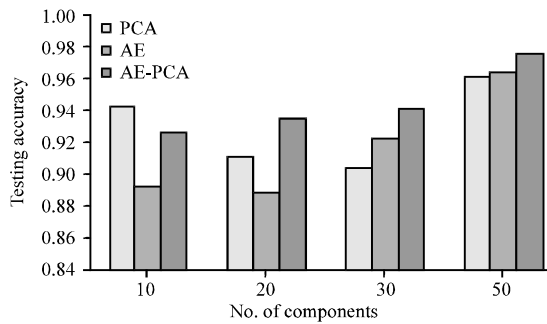
Fig. 12: Classification accuracy after dimensionality reduction for Pavia image
