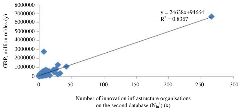
Fig. 4: Linear regression relationship between gross regional product (2007) and number of innovation infrastructure organisations in 80 regions of Russia (2007)
