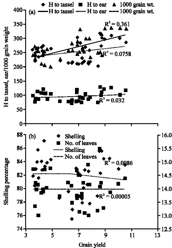
Fig. 1: Regression interdependence between grain yield, a) height to tassel, height to ear, 1000 grains weight and b) shelling percentage in control
