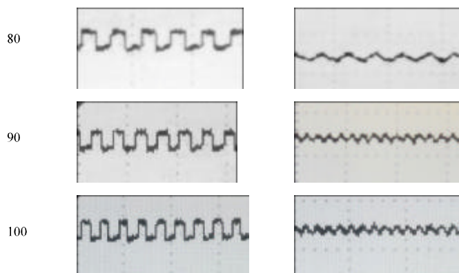
Fig. 12: The comparison of input and output signal as the frequency being increased up to 100 kHz
