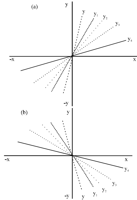
Fig. 7: Example of: a) Positives linear equation; b) Negative linear equation
