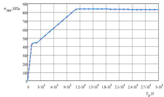
Fig. 6: Function of maximum von Mises stress depending on axial compressing force value (Results of computer simulation showed by labels and plotted function \sigma_{EQV} showed by solid curve)
