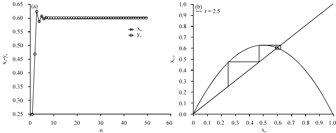
Fig. 2: Preimage of interval; a) logistic map, p = 2.5 and b) Spiderweb for logistic map
