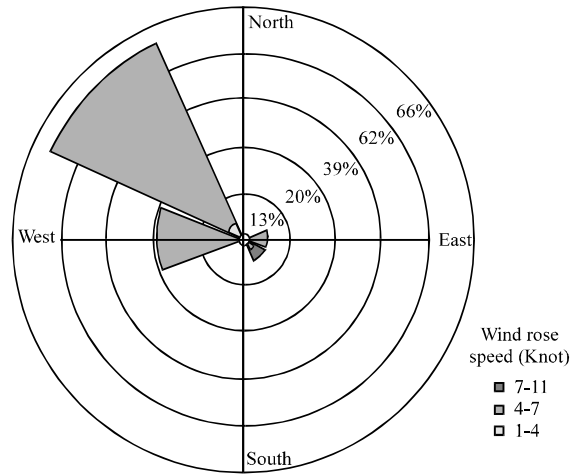
Fig. 1: Win rose in Makassar City year 2012-2016; Wind direction and speed
