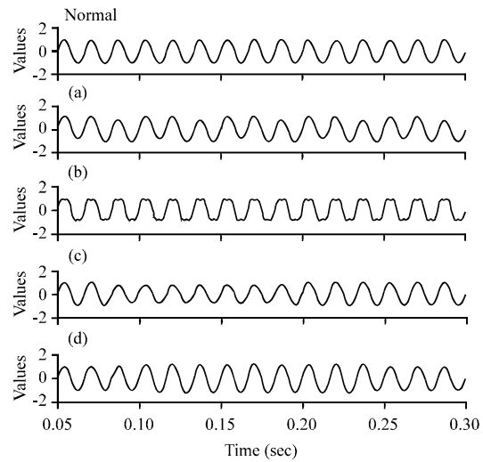
Fig. 6: Original normal waveform and its distortion signal; a) low frequency distortion; b) high frequency distortion; c) voltage sag from 0.08-0.196 sec and d) voltage swell. From 0.104-0.24 sec
