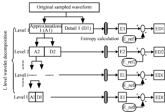
Fig. 5: Entropy-based features system architecture
