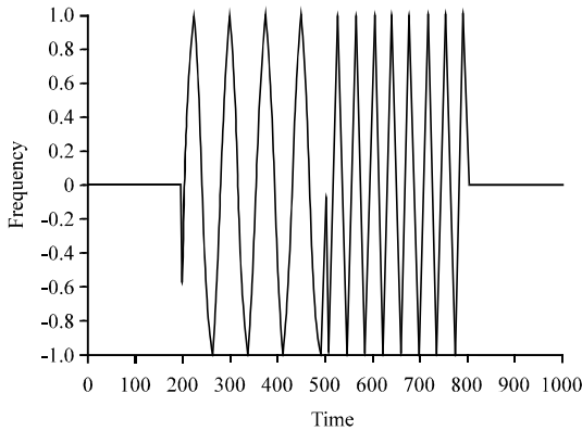
Fig. 3: Sinusoidal signal having two different frequency components at two different times
