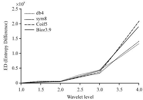
Fig. 12: Entropy-based features all wavelet method
