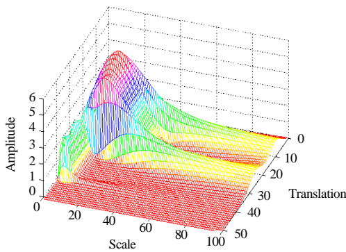
Fig. 4: Continuous wavelet transform of the sinusoidal signal
