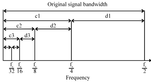
Fig. 8: The wavelet decomposition in the frequency domain
