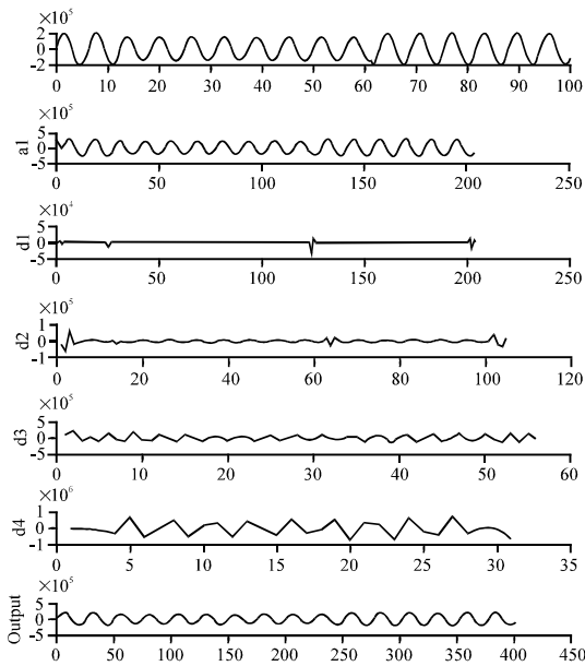
Fig. 9: 6.1 sag signal is applied on wavelet transform a1 is first level approximation coefficient d1, d2, d3 and d4
