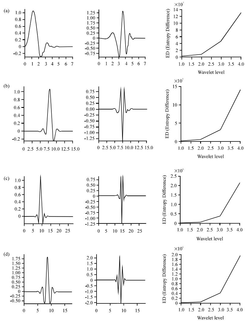
Fig. 10: Entropy-based features analysis; a) db4 wavelet scaling function and wavelet function-entropy-based features analysis result by db4; b) Sym8 wavelet scaling function and wavelet function-entropy-based features analysis result by sym8; c) Coif5 Wavelet scaling function and wavelet function-entropy-based features analysis result by coif5 and d) Bior3.9 wavelet scaling function and wavelet function-entropy-based features analysis result by bior3.9
