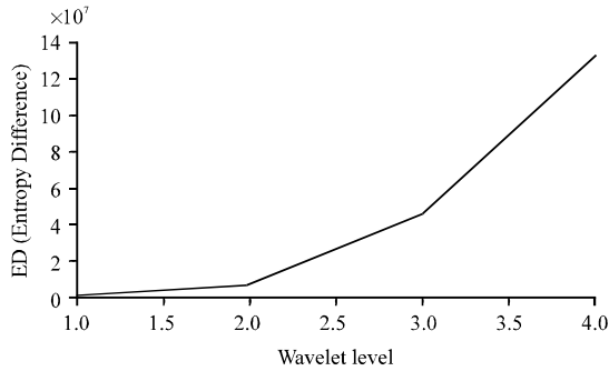
Fig. 11: Analysis result in band limited noise environment (SNR = 20 dB)
