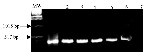
Fig. 2: Sensitivity of the PCR for detection of the 342 bp PCR product of RVFV from different strain of the virus. The RT-PCR detected different strains of RVFV. Molecular weight marker (100 bp DNA ladder); Lane (1-6): RVFV RNA extracted from RVFV infected Vero cells and serum samples. Lane 1: RVFV RNA extracted Smith burn vaccine strain grown on Vero cells (positive control); Lane 2-3: RNA extracted RVFV strain grown on Vero cells; Lane 4-5: RVFV RNA extracted from human serum samples. Lane 6: RVFV RNA extracted from spleen sample of infected goat; Lane 7: total nucleic acid extracted from non-infected Vero cells (negative control)
