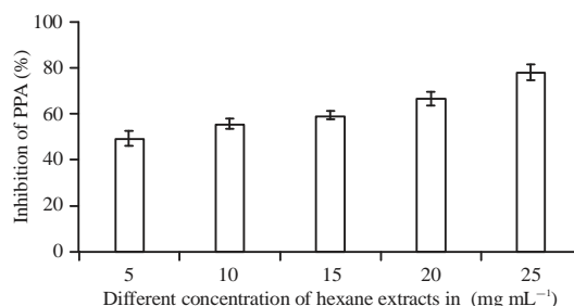
Fig. 1: Inhibition of PPA by n-hexane extract. Increasing concentration was pre-incubated with PPA at 37°C for 10 min
