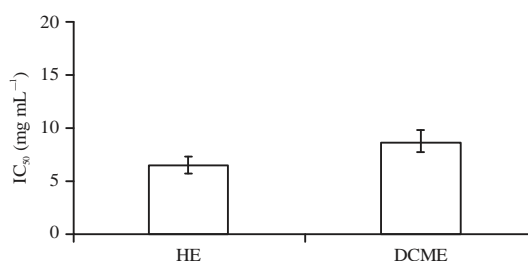
Fig. 3: IC_{50} values of n-hexane (HE) and dichloromethane (DCME) extracts
