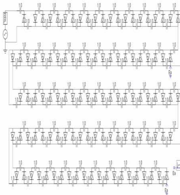
Fig. 7: Proposed 15kV DC power supply simulation circuit by PSCAD simulation works
