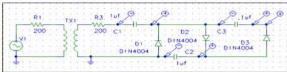
Fig. 4: Connection diagram half-wave voltage tripler.
