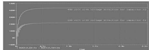
Fig. 8: Simulation result of the voltage doubler circuit by PSpice
