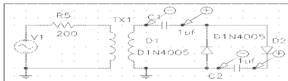
Fig. 1: Connection diagram half-wave voltage doubler
