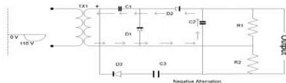
Fig. 6: Voltage tripler in negative alternation
