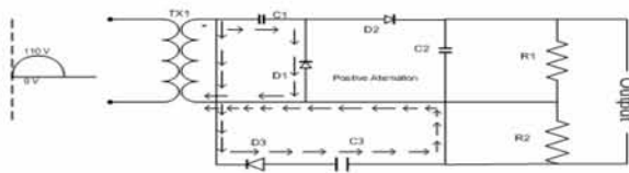
Fig. 5: Voltage tripler in positive alternation
