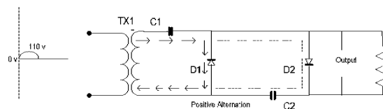
Fig. 2: Voltage doubler in positive alternation
