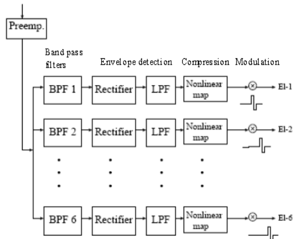
Fig. 2: Block diagram of the CIS strategy
