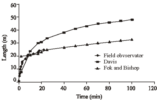
Fig. 5: Graphs of observed and computed rates of advance of water in furrows of sandy loam at Q = 1.8l/s and slope 0.6%
