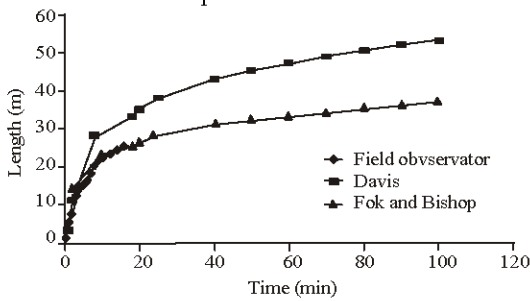
Fig. 6: Graphs of observed and computed rates of advance of water in furrows of sandy loam at Q = 2.0L/S and slope 0.6%
