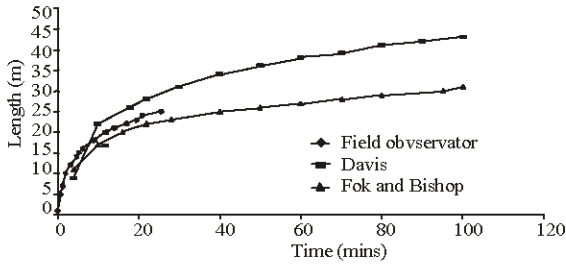
Fig. 4: Graphs of observed and computed rates of advance of water in furrows of sandy loam at Q = 1.6l/s and slope 0.6%
