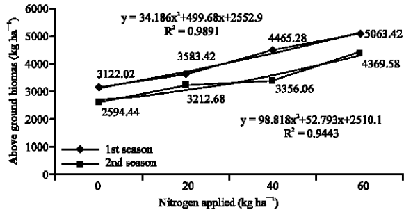
Fig. 2: Effect of nitrogen on total above ground biomass of chickpea (kg ha -1 ) at harvest in seasons I and II at Naivasha
