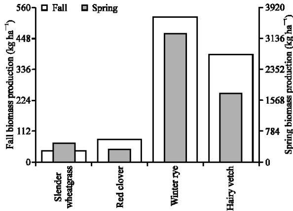
Fig. 4: Individual cover crop biomass production; fall biomass growth from planting until killing frost; spring biomass growth from early spring until herbicide burndown approximately two weeks before planting for the 2002 experiment
