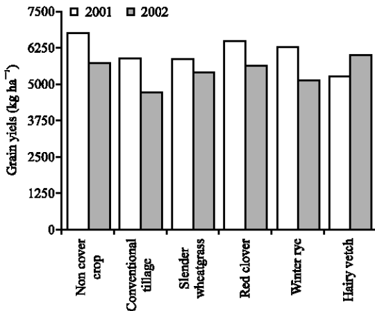
Fig. 5: Corn yield following cover crop growth for each treatment for the 2001 and 2002 growing seasons
