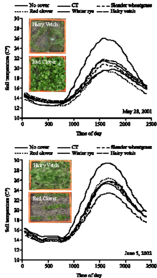
Fig. 1: Soil temperature at 7.5 cm for the day following planting for select cover crop treatments, Brookings, SD 2001 and 2002
