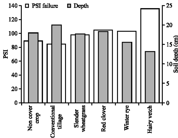
Fig. 3: Soil bearing strength pressure and the depth of soil failure, by treatment for the 2002 experiment
