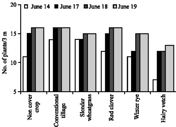
Fig. 2: Stand establishment counts, number of plants emerged in three meter of row, by treatment for the 2002 experiment
