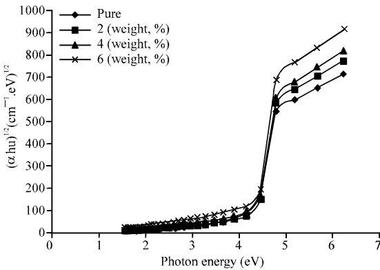
Fig. 3: Relationship between (\alpha hu)^{1/2} ( \text{cm}^{-1} \cdot \text{eV} ) 1/2 and photon energy of PS-WBP composites
