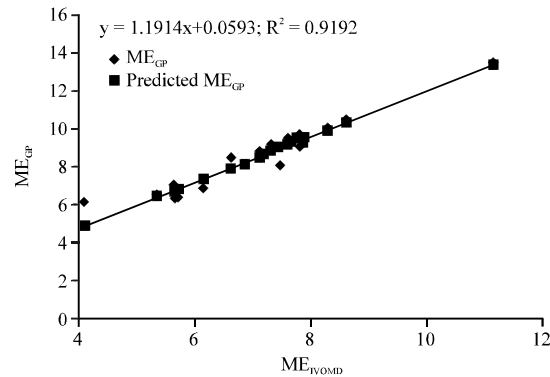
Fig. 3: Linear relationship between ME estimated from in vitro digestibility ( ME_{IVOMD} ) and ME by Menke gas systems ( ME_{GP} )
