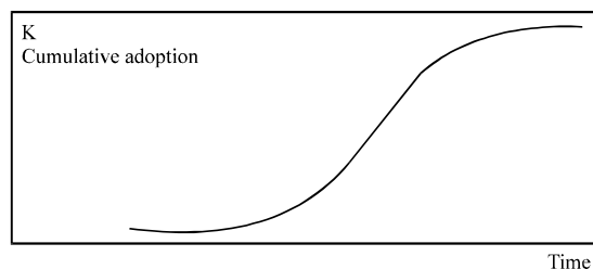
Fig. 1: Logistic regression
