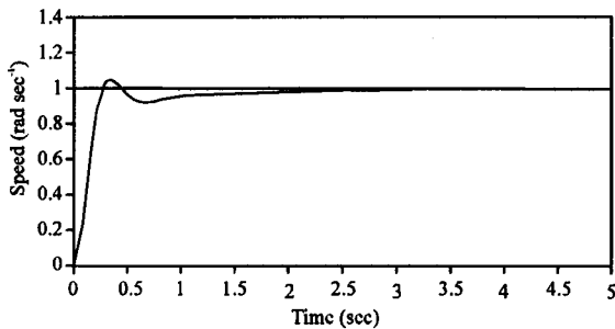
Fig. 10: Step response of DC motor with optimum PI-controller parameters for given specifications
