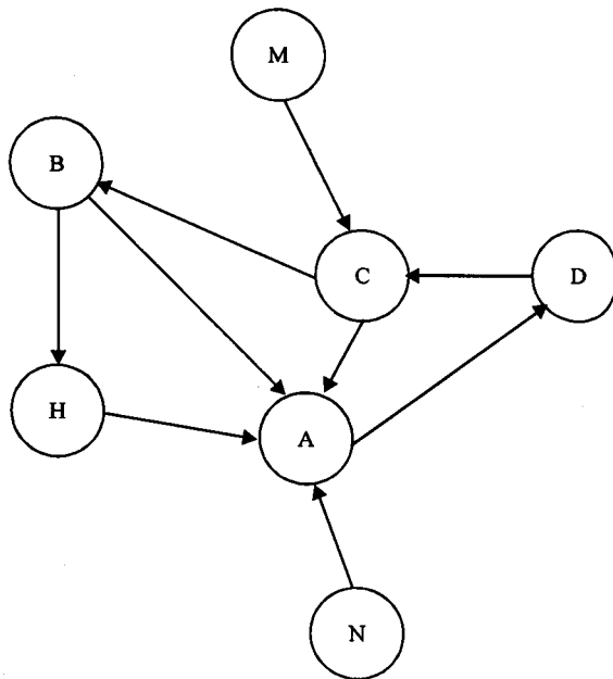
Fig. 2: Directed graph reflect the dependency between modules
