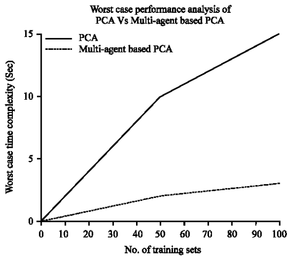
Fig. 4: Performance analysis
