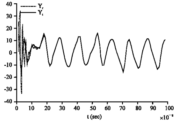
Fig. 7: The synchronization recovery with the compensator
