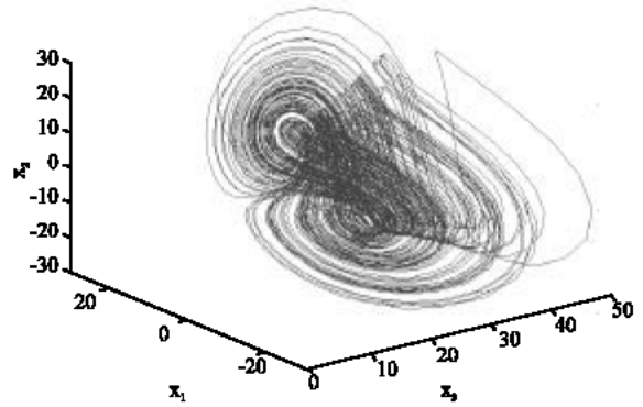
Fig. 1: The typical Chen Chaotic attractors
