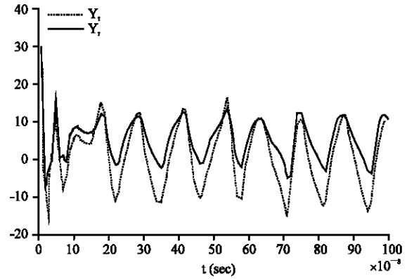
Fig. 3: Synchronization between transmitter and receiver in satellite channel with attenuation A = 2 and offset B = 6
