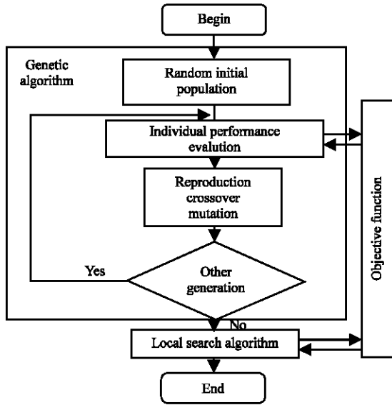
Fig. 5: Flowchart of genetic algorithms
