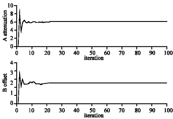
Fig. 6: Estimation the values of attenuation and offset
