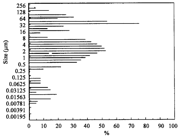
Fig. 2b: Incremental pore volume vs. Pore diameter (at 800°C - 850 °C)
