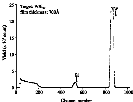
Fig. 2: RBS spectra of sputtered film from a WSi_{2.7} composite target
