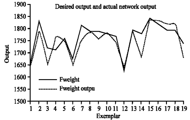
Fig. 3: GFFNN results
