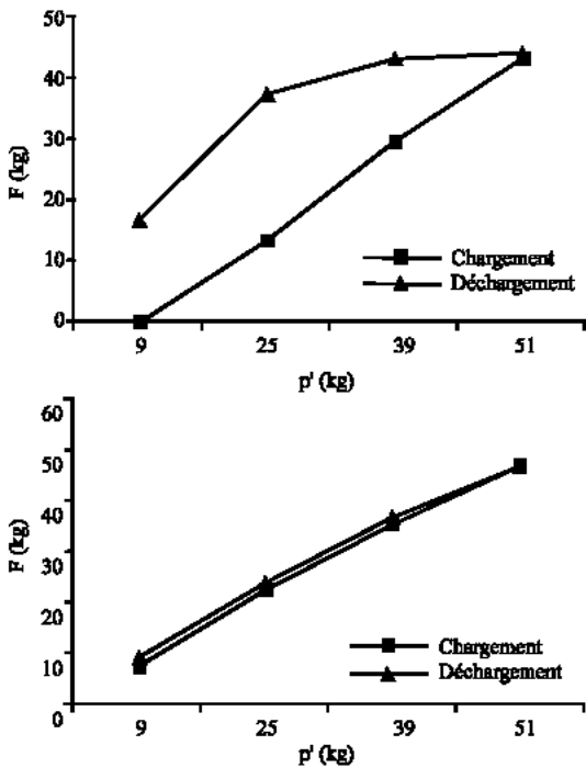
Fig. 3: Calibration forces
