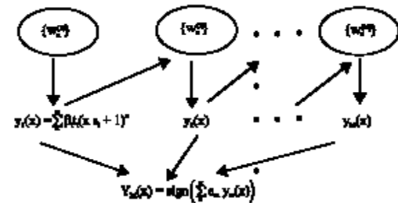
Fig 3: Schematic illustration of the K-Boosting framework
