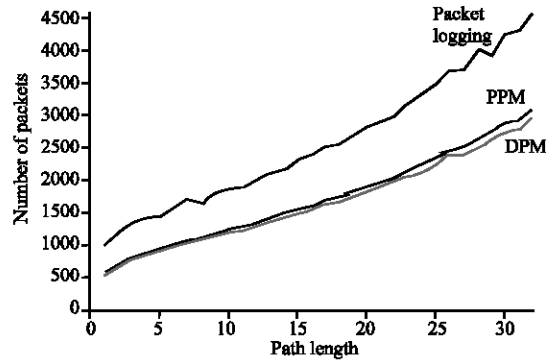
Fig. 8: Experimental results for number of packets required for path reconstruction with marking probability set at 1/25
