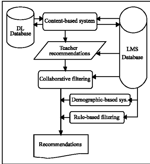
Fig. 2: A general proposal structure of RS algorithm
