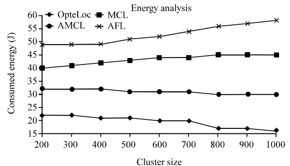
Fig. 1: Cluster size vs. consumed energy
