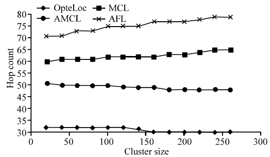
Fig. 7: Cluster size vs. avg hop count
