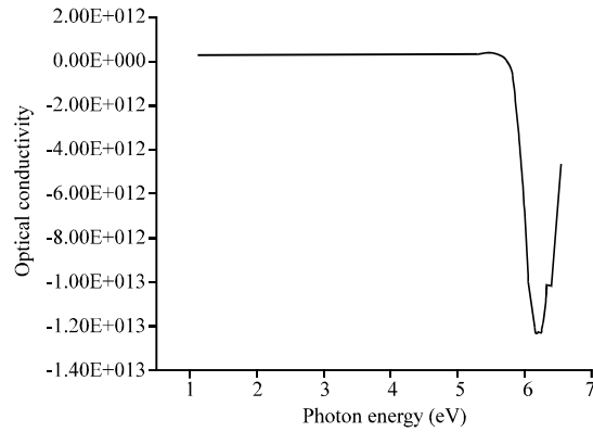
Fig. 6: Photon energy versus optical conductivity in GLO crystal
