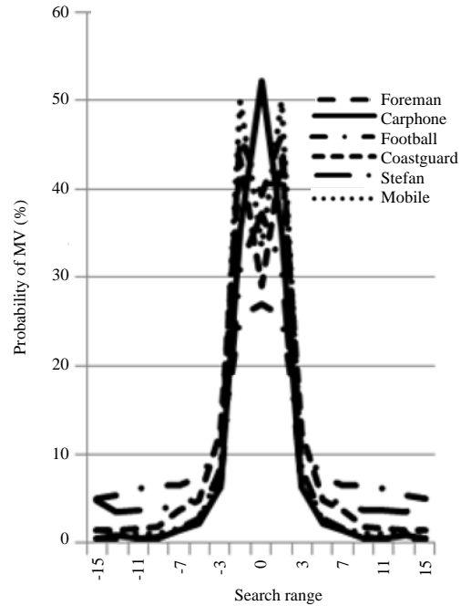
Fig. 1: Motion vector distribution for various video sequences
