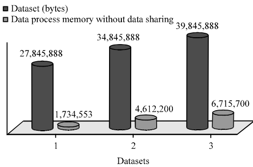
Fig. 6: Process memory consumption after ONT
